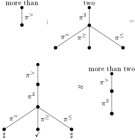
Fig. 7. Sequential composition of ‘more than’ and ‘two’
